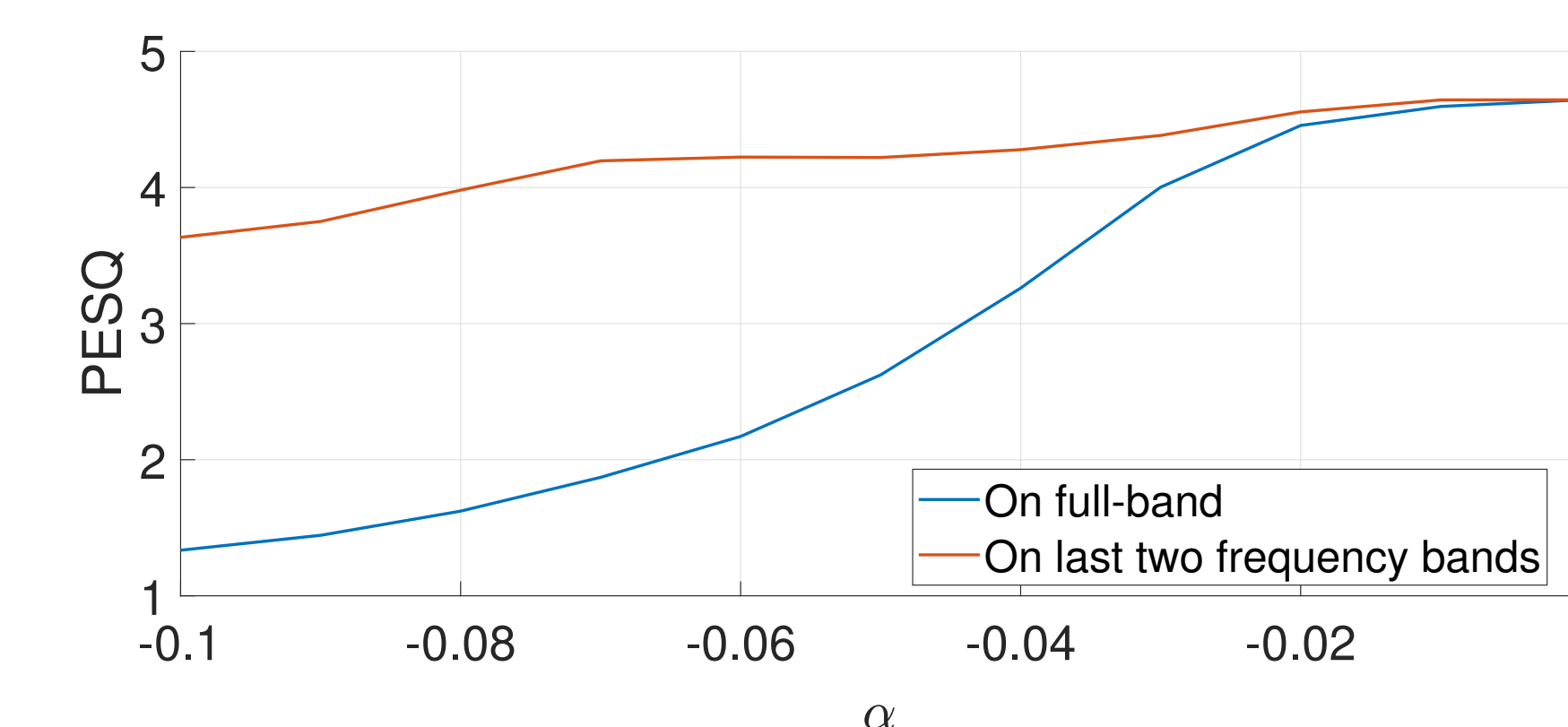
Figure 5: PESQ of freping output vs. warping parameter \alpha . Freping only in the higher bands causes less degradation in speech quality. HAs tend to resonate at higher frequencies due to feedback.
