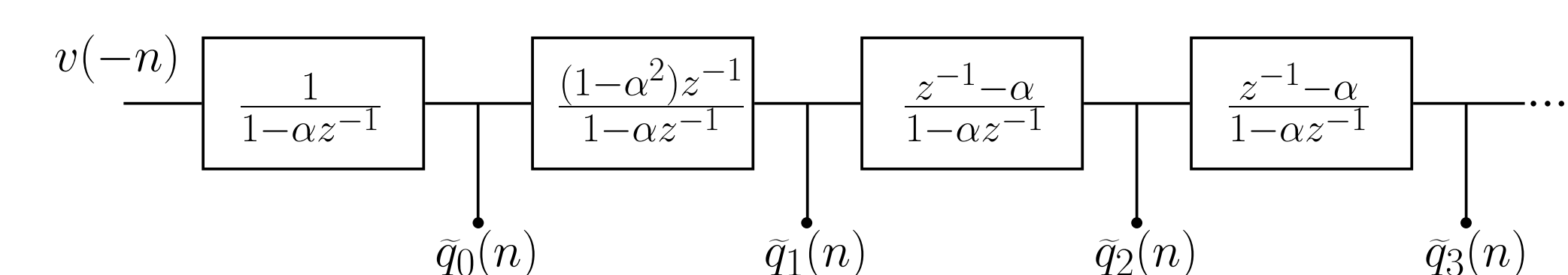
Figure 1: The all-pass network for frequency warping. The time-reversed signal v(-n) is first passed through the network and then q(k) is given by sampling \hat{q}_k(n) along the cascade chain at n = 0 , i.e., q(k) = \hat{q}_k(0) [1].
